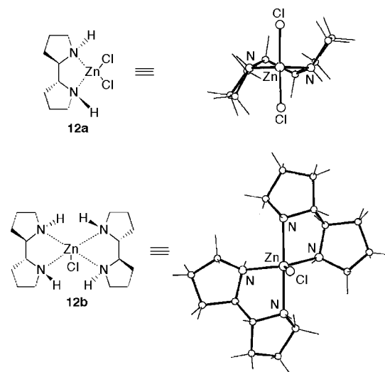
Figure 3. X-ray structures of 12a and 12b , the complexes formed between 2,2'-bipyrrolidine ( 9 ) and \text{ZnCl}_2 .
